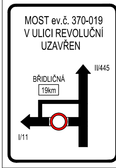
DETAIL "B"–IS11a
